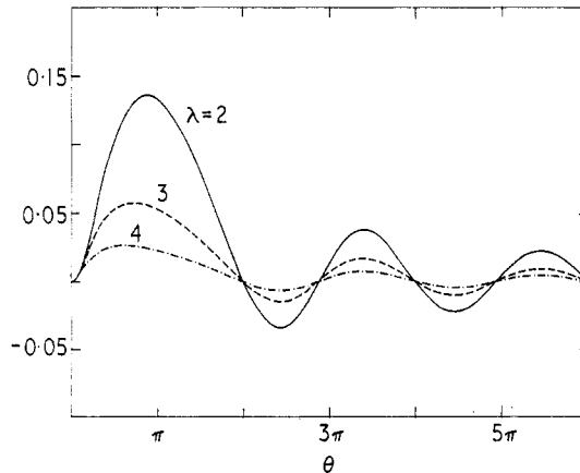
Figure 3. The ion contribution to the normalized sheath conductance G_1/(\epsilon_0\Pi_1^2/c) against the transit angle \theta of the ion in the sheath. The plotted curves are labelled with the value of the parameter \lambda .
